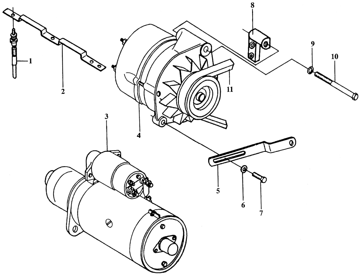
Fig. 12 Electric System Assy(Y385Y-1)
