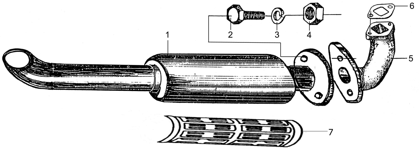
Fig. 13 Silencer Assy(Y385T-1)
