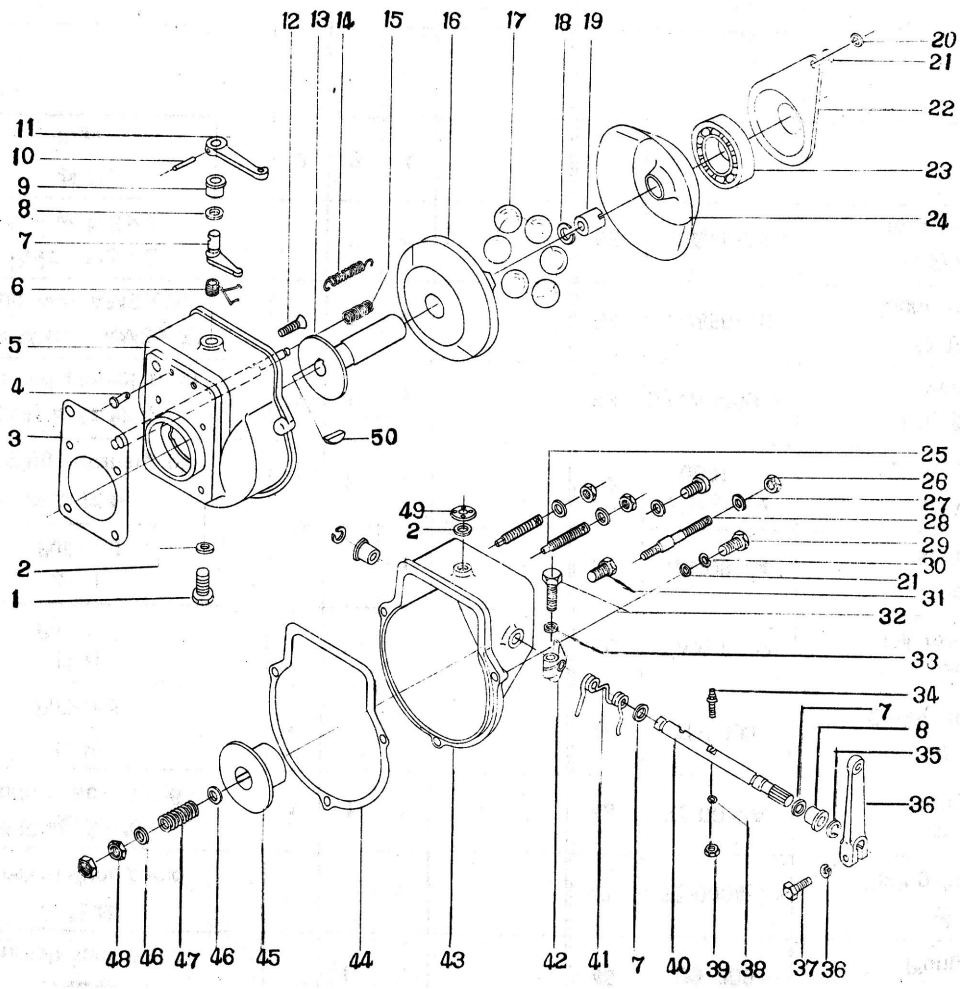
Fig.017 Speed Governor Assy
