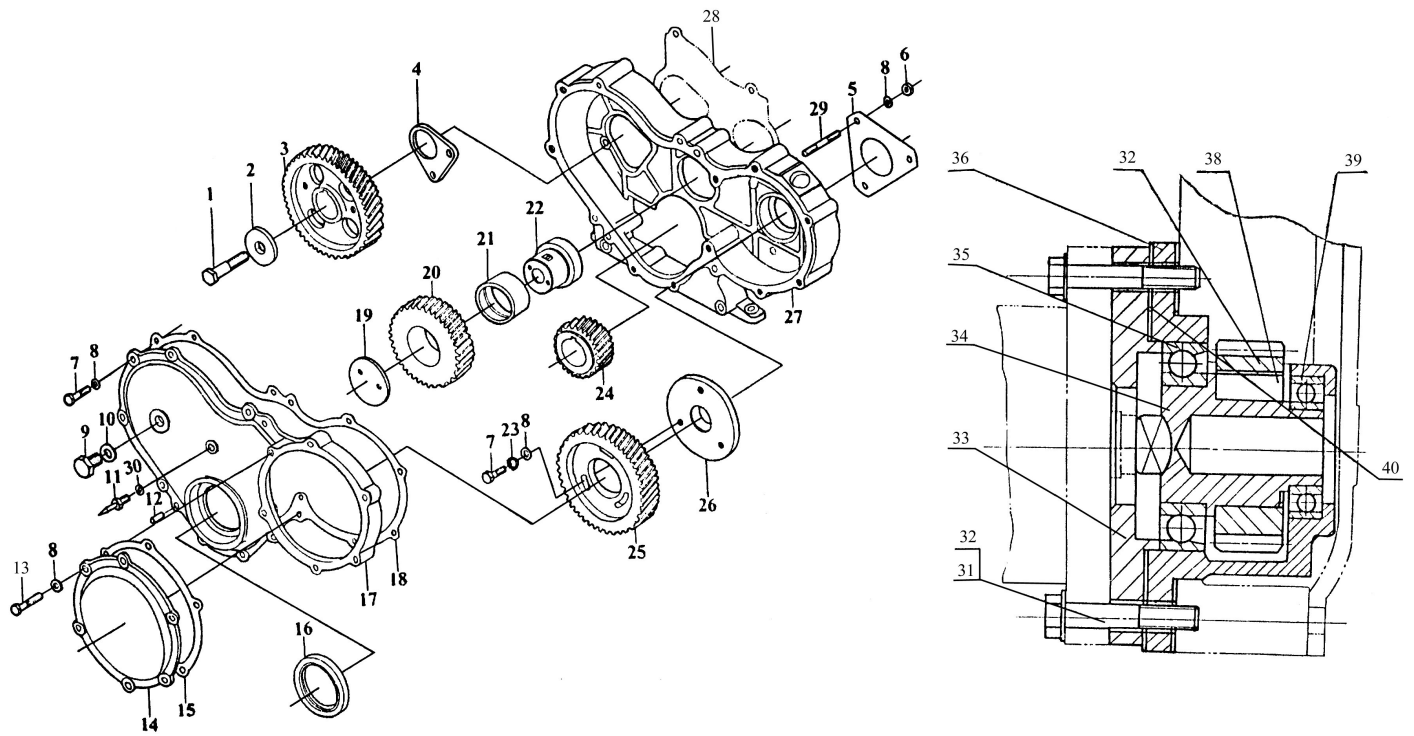
Fig. 2 Timing Gear Case Assy (Y3851-1)
